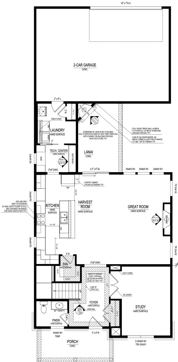
Main Level
