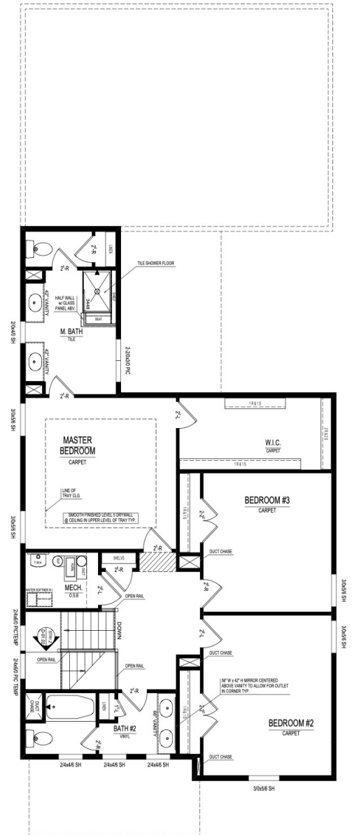
Upper Level
