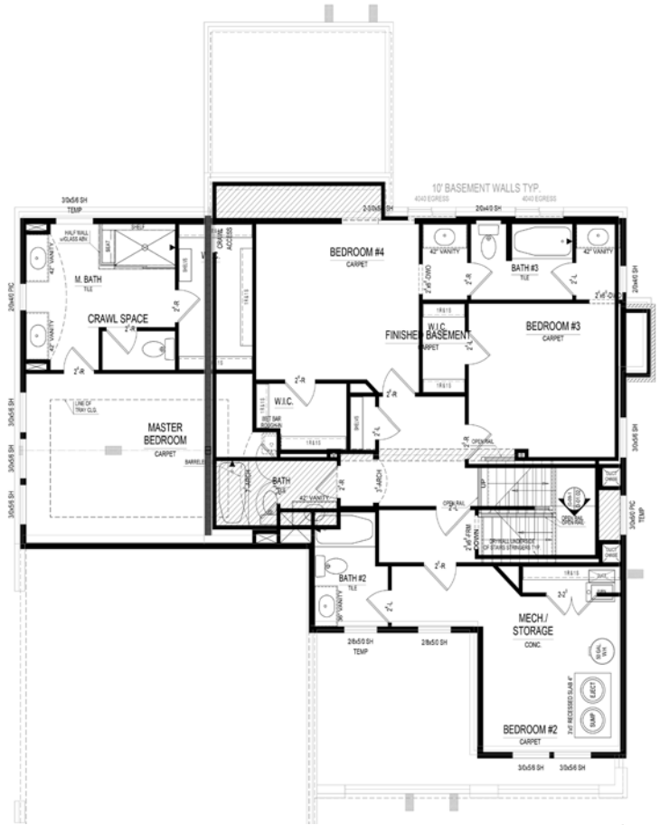
Upper Level
