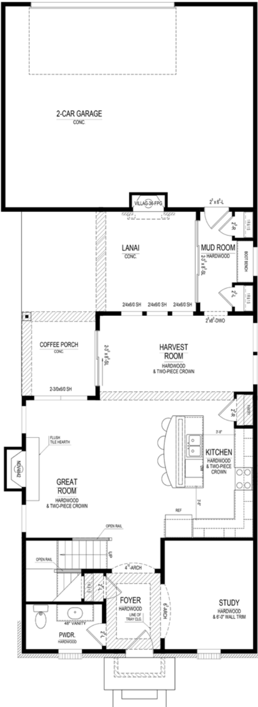
Main Level
