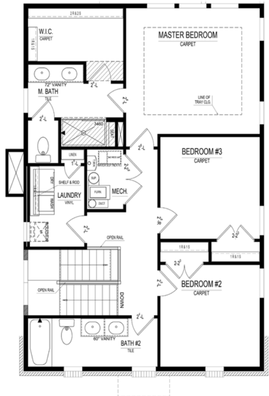
Upper Level
